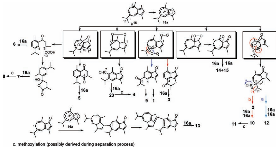
Scheme 1. Biogenetic Relationship of the Isolated Compounds
