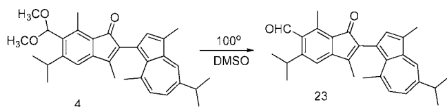
Figure 3. Conversion of 4 to 23.
