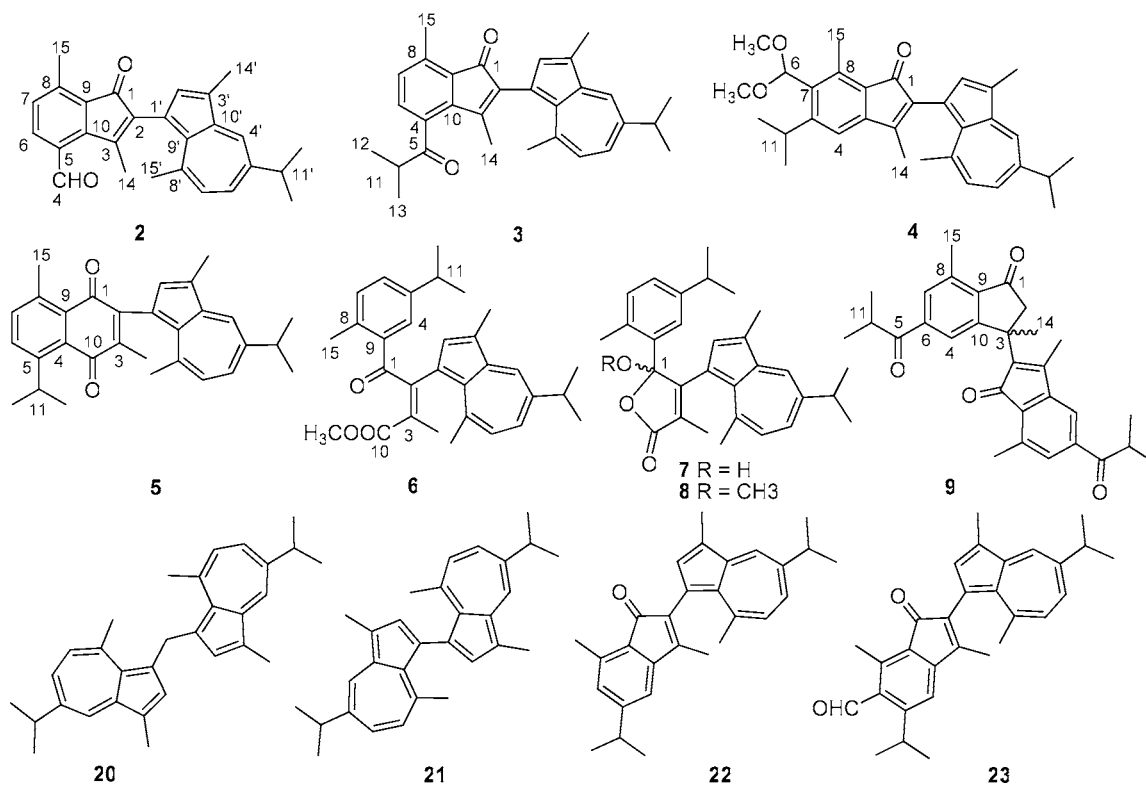
Figure 2. Structures of anthogorgienes B–I (2–9) and known dimers.
